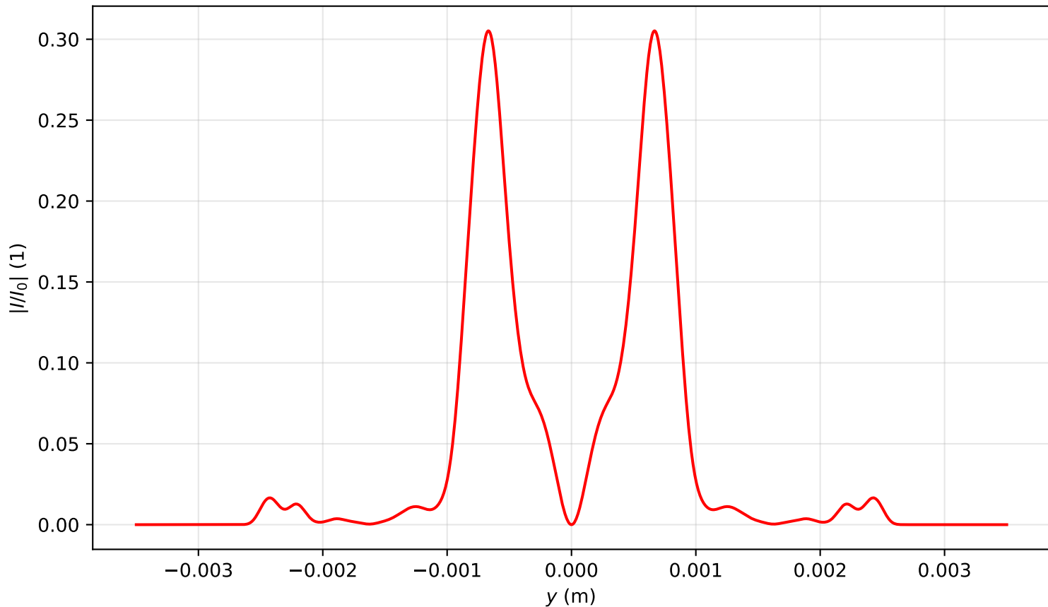
Intensity profile I(x=0, y, z=1.990)/I_0 , \text{Pin}=8.0\text{Pcr} , artificial time
